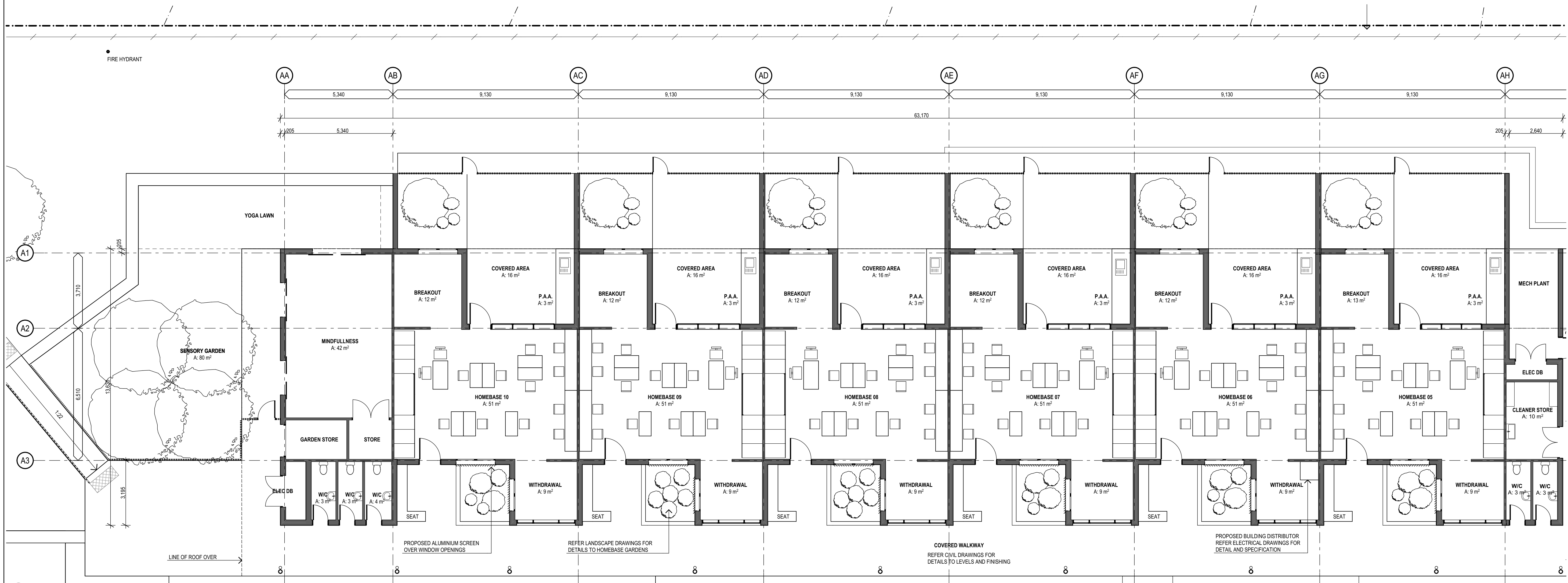
1 DETAILED PLAN 1:100
